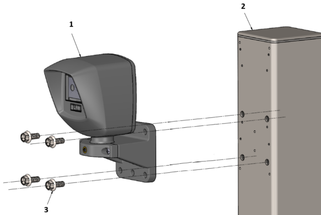
1: IRB-RET-2 or MRD-1P, 2: 325-POST-2, 3: MOUNTING SCREW
