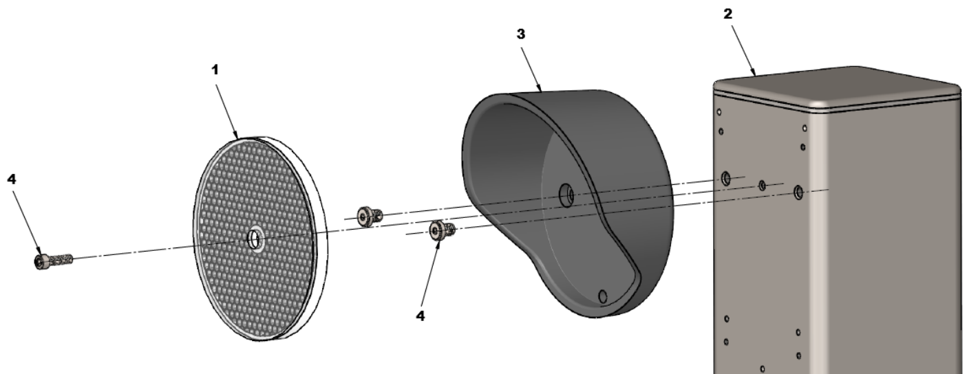
1: REFLECTOR, 2: 325-POST-2, 3: REFLECTOR HOOD, 4: MOUNTING SCREWS
