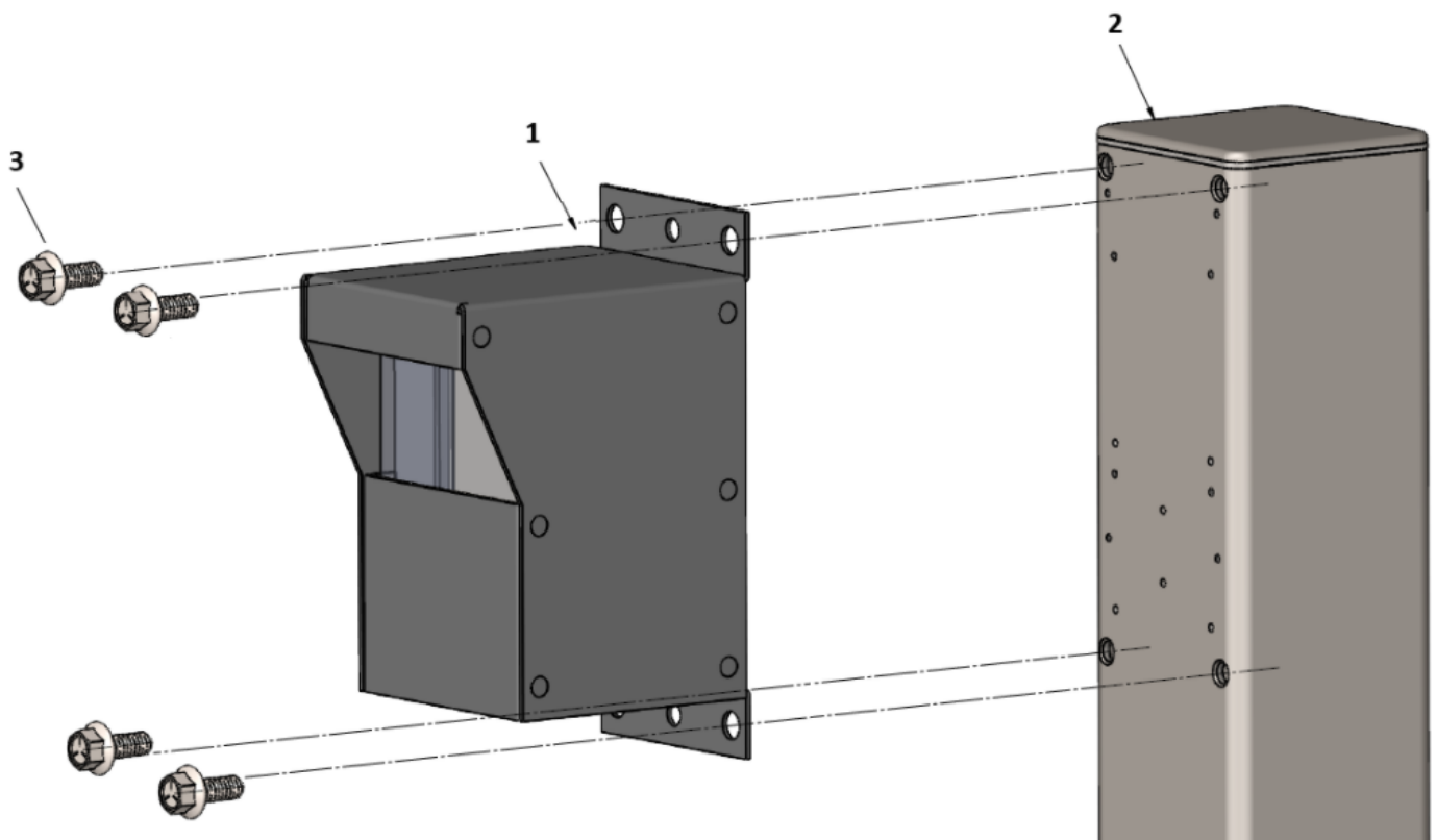
1: IRB-325-2 (under Hood), 2: 325-POST-2, 3: MOUNTING SCREW
