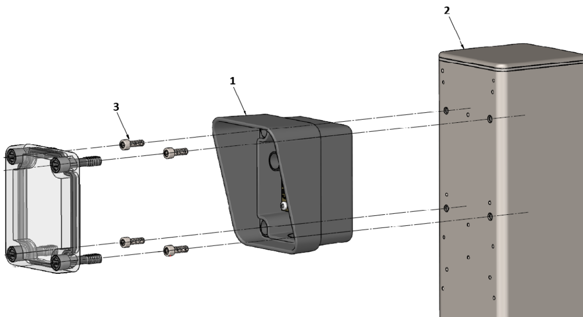
1: IRB-MON-2, 2: 325-POST-2, 3: MOUNTING SCREW
