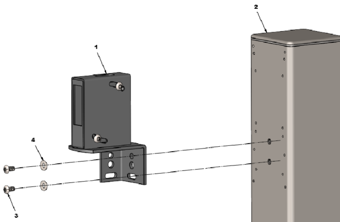
1: NIR-50-325 (under Hood), 2: 325-POST-2, 3: MOUNTING SCREW 4: WASHER
