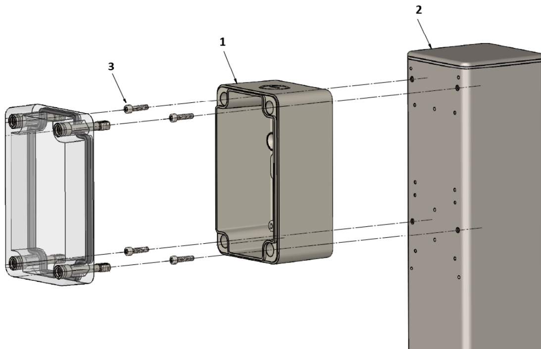
1: IRB-325-2, 2: 325-POST-2, 3: MOUNTING SCREW
